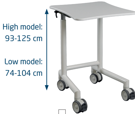
FlexVan W: 55, D: 60 cm Prod. No. 18-807001H/L-OX
